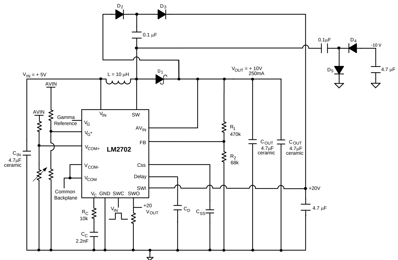
Figure 46. 5V to 10V TFT Application
